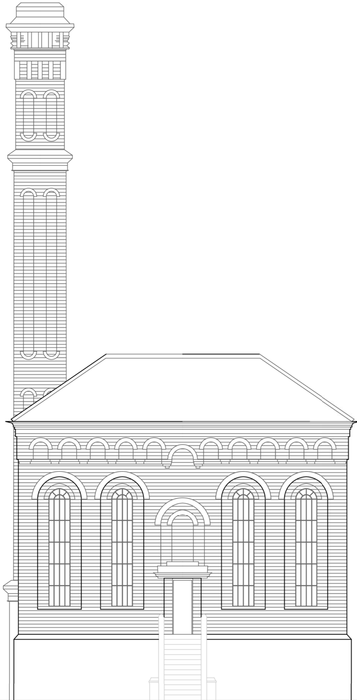
WEST ELEVATION @SCALE 1:100
